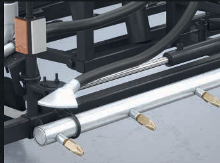
The swivelling wash piping is equipped with fan nozzles and lateral shift.
